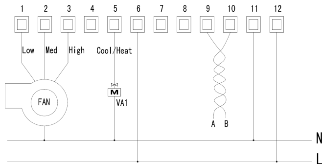
LCF Touch Modbus – Manual mode wiring diagram for 2-pipe fan coil
