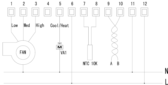
LCF Touch Modbus – Auto mode wiring diagram for 2-pipe fan coil
