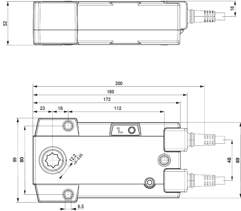
Dimensional drawings
