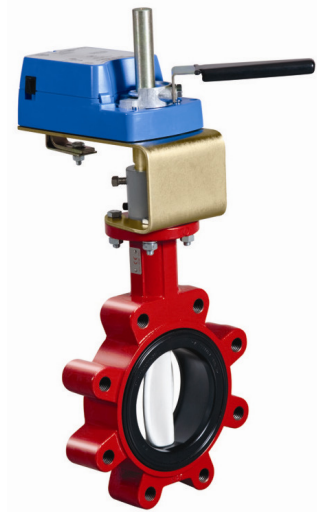
Two-Way Valve with M9000 Series Non-Spring-Return Electric Actuator (without Weather Shield)
