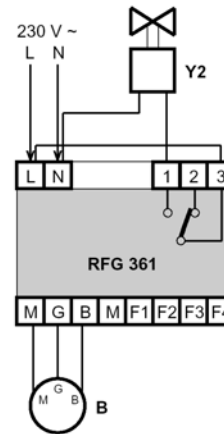
Solenoid valve N/C:
