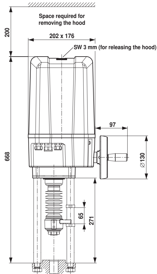
Dimensional drawing
