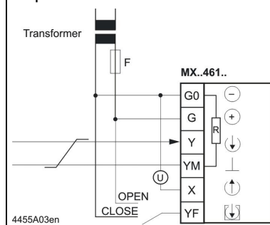
Separate transformer
