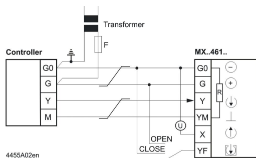
Common transformer
