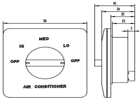
Dimension diagram
