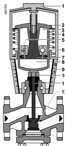
Valve open
