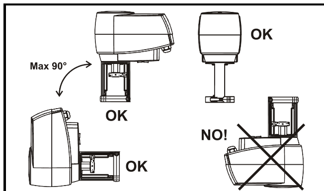
Figure 5: mounting positions
