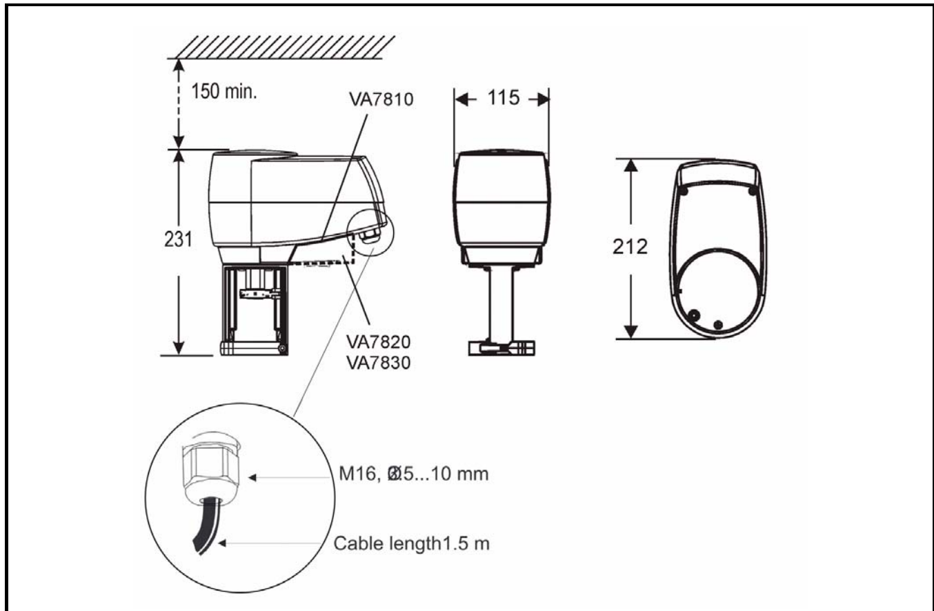
Figure 9: dimensions
