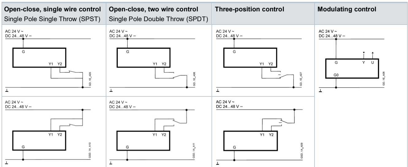
GLB1.. 1E (AC 24 V ~ / DC 24...48 V ~)
